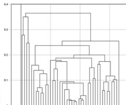
Dendrogram. Hierarchical clustering.
